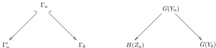
FIGURE 1. Inclusions of lattices (left) and coverings of complexes of groups (right)
