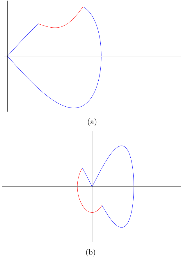
Figure 13. (a) An asymmetric orbit with P \geq 1 and Q = 0 . (b) An asymmetric orbit with P = 2 and Q = 1 .
