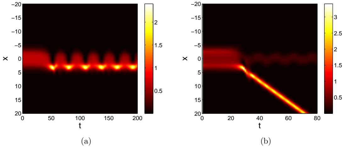
Figure 4. Time dynamics of solutions at points indicated as B and C in Fig. 2. Shown is the top view of |\Psi(x,t)|^2 .
