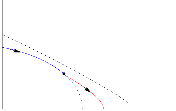
Figure 8. Part of an unstable orbit that appears when the heteroclinic orbit of the inner system (the black dashed line given by equation (14) - colour online) is ‘close’ relative to the homoclinic orbit of the inner system (the blue dashed line given by equation (13)). The dot represents the jumping off point. The black arrows represent the direction of travel in the phase plane. The orbit follows first the blue curve and then jumps to the red curve. As \frac{\omega}{V} decreases the blue dashed line will cross the black dashed line and unstable orbits of the second type will appear (See figure 9(b) for an example of such an orbit).
