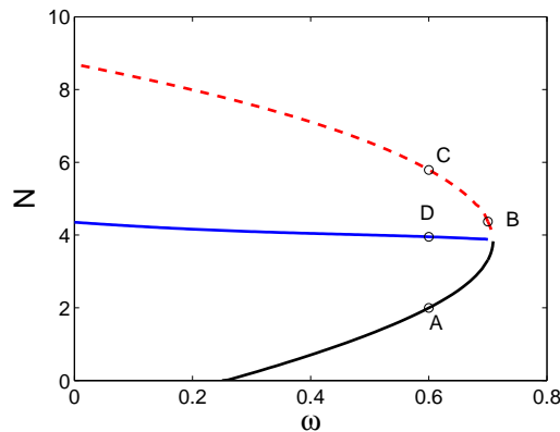
Figure 2. (Color online) The norm N as a function of \omega for the first (positive) state corresponding to the first branch in Fig. 1. As \omega increases from the bifurcation point \omega \approx 0.265 , there is a bifurcation at which the state becomes unstable. In addition to the symmetric positive states, there is also a stable asymmetric state along the middle (solid blue) branch. Solid and dashed curve represents stable and unstable solutions, respectively.
