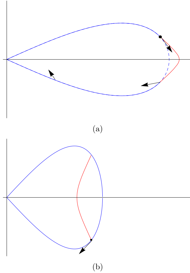
Figure 9. (a) An unstable orbit of the first type. The dashed line is the homoclinic orbit of the outer system. The dot represents the jumping off point. The black arrows represent the image of a tangent vector to a solution under the variational flows \Phi^{O,I} at various values. (b) An unstable orbit of the second type. The dot represents the jumping off point. The black arrow represents where \Phi(\mathbf{b}^O) stops being tangent to the orbit of the solution.
