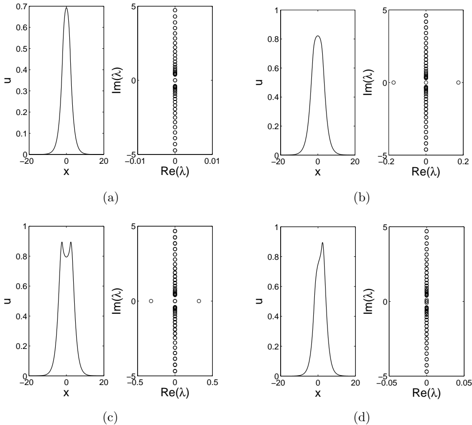
Figure 3. Profile of solutions at points indicated as A–D in Fig. 2 and their eigenvalue structures in the complex plane. The phase-portraits of the solutions in each panel are presented in Fig. A1.
