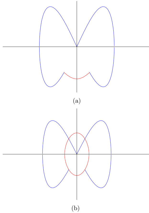
Figure 11. (a) An unstable orbit where P = 3 and Q = 1 . (b) An unstable orbit where P = 2k + 3 and Q = 2k + 1 and k \geq 1 . The number k describes the number of periods the solution stays in the inner periodic orbit.
