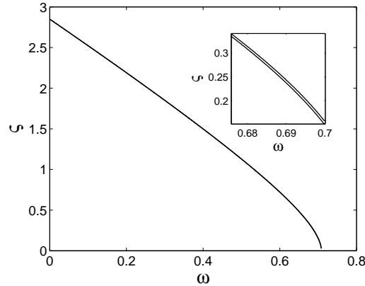
Figure 10. The spectrum \zeta > 0 of D_+ for unstable symmetric solutions along the upper branch in Fig. 2 as a function of \omega . The inset zooms in on a small region clearly showing that there are two curves.
