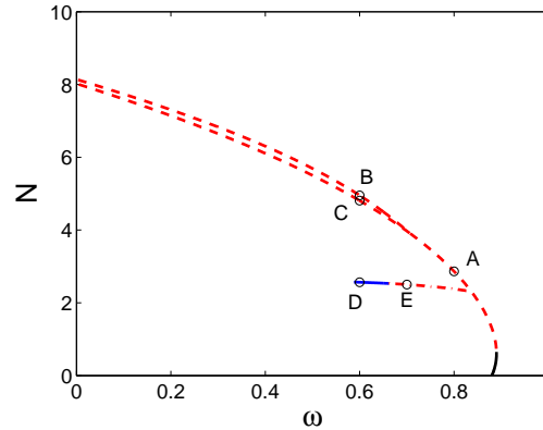
Figure 5. The same as Fig. 2, but for the first excited state, corresponding to the second branch in Fig. 1. The bifurcation point of the linear state is \omega \approx 0.898 .
