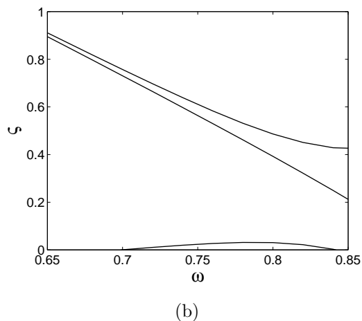
Figure 12. (a) A sketch of symmetric orbits with P \geq 2 and Q = 1 . (b) The same as in Fig. 10, but for unstable symmetric solutions in Fig. 5.
