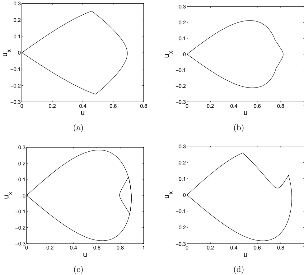
Figure A1. Phase portraits of solutions at points indicated as A–D in Fig. 2 (see also Fig. 3).
