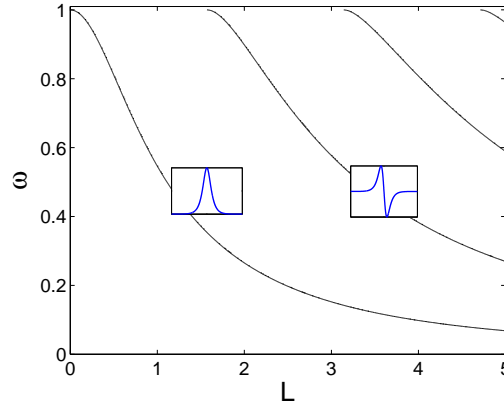
Figure 1. Bifurcation points of non-uniform solutions from the zero solution u \equiv 0 in the (L, \omega) -plane for V = 1 . The insets present a sketch of the corresponding solution u(x) along the first two branches.
