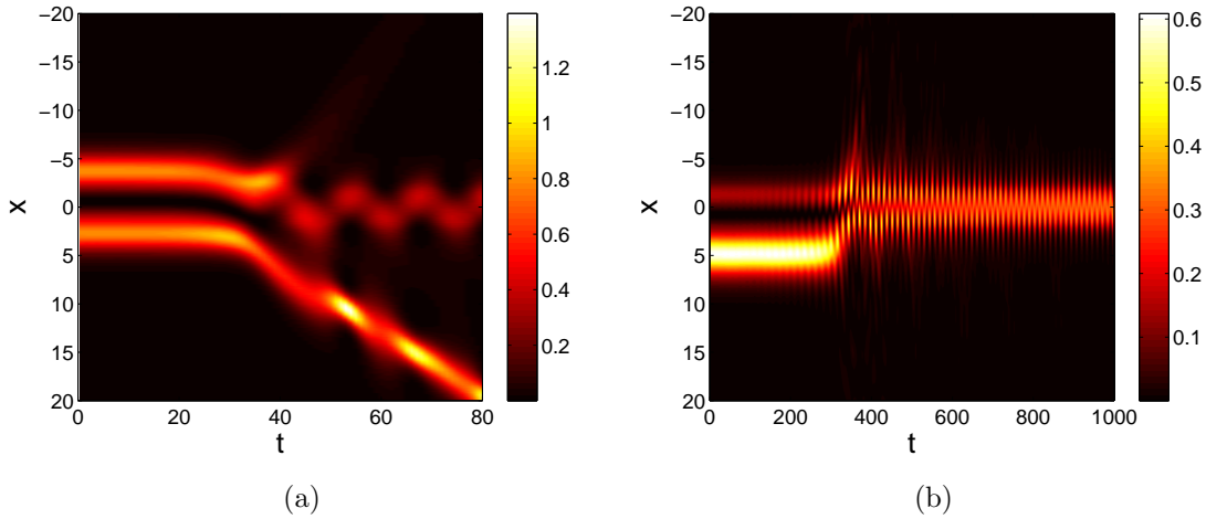
Figure 7. The dynamics in time of solutions at points indicated as B and E in Fig. 5, respectively. Shown is the top view of |\Psi(x, t)|^2 .
