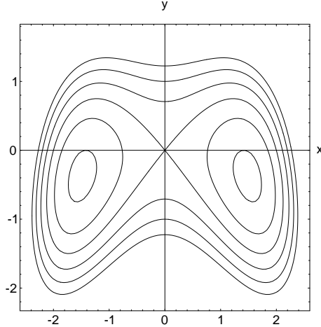
Figure 3. The equipotential lines V = -0.5, 0, 0.5, 1, 1.5 for a = 1 , \varepsilon = 1/3 in (22). In the integrable case \varepsilon = 0 there are two stable periodic orbits parallel to the y -axis crossing the minima at y_0^2 = -\varepsilon x_0^2 , x_0^2 = a/(1 - 2\varepsilon^2) . The critical energy of the minima is a^2/(8\varepsilon^2 - 4) , for the saddle point at the origin it is 0. The unstable orbit crossing the saddle moves on the y -axis for all values of \varepsilon . It is also part of the tangent set of the section \dot{x} = 0 . There are homoclinic orbits associated with this orbit that intersect the section only once and then approach the invariant part of the tangent set for t \rightarrow \pm\infty .
