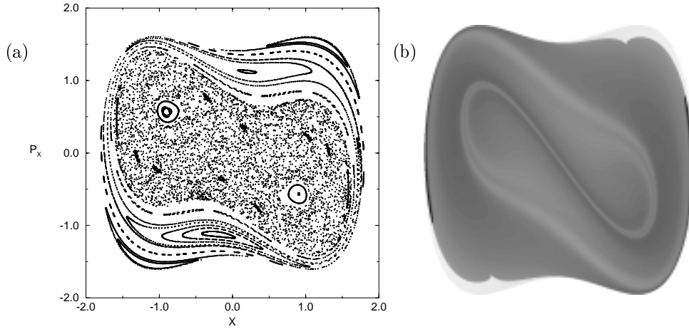
Figure 6. The W -section \dot{p}_y = 0 for (22) with \varepsilon = 0.1 , a = 1 and h = 1 . After a canonical point transformation Y = V_y = y + \varepsilon x^2 , X = x , the projection of \Sigma_w onto the plane (X, P_X) = (x, p_x - 2\varepsilon xp_y) with \ddot{p}_y > 0 gives a canonical representation of P on \mathbb{R}^2 which is used here. In (a) some orbits of the Poincaré map P are shown. In (b) the return time \tau is illustrated. Dark grey corresponds to large return times. The maximum return time is \approx 10 , i.e. the section is \Sigma -complete. Because the tangent set (which corresponds to the boundary of the shown projection of \Sigma_w ) is not invariant, P is discontinuous along the preimage of \Omega , as can be seen in the upper right and in the lower left part of (b), where there is a jump in the grey scale. Although P is discontinuous, invariant tori intersecting the section continue smoothly across the discontinuity as can be seen in (a). The two islands embedded in the chaotic sea correspond to the stable orbits that are lost in the incomplete section shown in figure 4.
