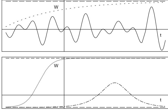
Figure 2. (a) Types of signals for a function W : the solid line shows the generic case of a signal, which repeatedly has extrema, the dashed line indicates the signal of an orbit which lies entirely in the section and the dotted line shows the signal of an orbit asymptotic to the previous one in forward time. (b) Schematic signal of homo- and heteroclinic motion: the two dashed lines represent unstable periodic orbits, which lie entirely in the section; heteroclinic motion can be identified as the dotted line while the remaining line stands for homoclinic motion. Notice that the sketch represents worst case, non-winding periodic orbits. The approach to a winding orbit would give a signal which oscillates an infinite number of times around its final value.
