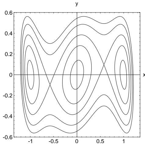
Figure 5. The equipotential lines 27V = 0.5, 2, 3.75, 6, 8 for \varepsilon = 1/2 in (24). In the integrable case \varepsilon = 0 there are three stable periodic orbits parallel to the y -axis crossing the minima at x = 0, \pm 1 on the x -axis. The potential minima are 0, while the saddle points have V = (4 - \varepsilon^2)/27 . The perturbation is chosen in such a way that the two unstable orbits crossing the saddles at x_0 = \pm 1/\sqrt{3}, \pm y_0 = \varepsilon x/3 keep moving parallel to the y -axis if \varepsilon \neq 0 . These orbits are part of the tangent set of the section \dot{x} = 0 . There are heteroclinic orbits connecting them that do not intersect the section but only approach the invariant part of the tangent set for t \rightarrow \pm\infty .
