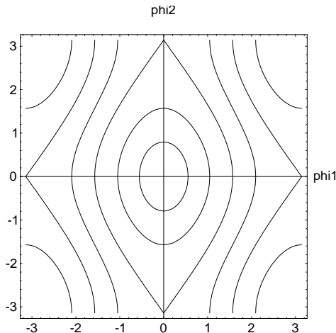
Figure 7. The equipotential lines V = 0.5, 1, 2, 3, 4, 5 for the mathematical double pendulum, i.e. \alpha = 2 , \beta = 1 , \gamma_1 = 2 , \gamma_2 = 1 in (28). The critical energies correspond to the origin ( h = 0 ), the cusps on the \phi_2 -axis ( h = 2 ), the cusps on the \phi_1 -axis ( h = 4 ) and the four corners of the picture ( h = 6 ), which are identified to one point on the torus. Because the kinetic energy depends non-trivially on q , there are no periodic orbits along the symmetry lines of the potential.
